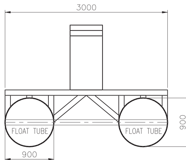
SECTION VIEW
