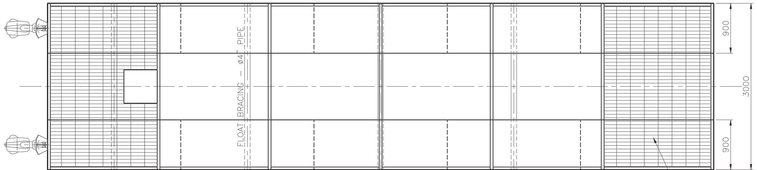
PLAN ON MAIN DECK
